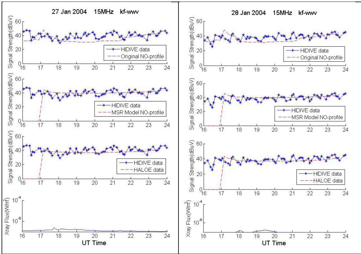
Figure F.7. HIDIVE data, GOES data, and AbbyNormal version predictions for the 15 MHz kf-wwv transmission on 27 January 2004.
