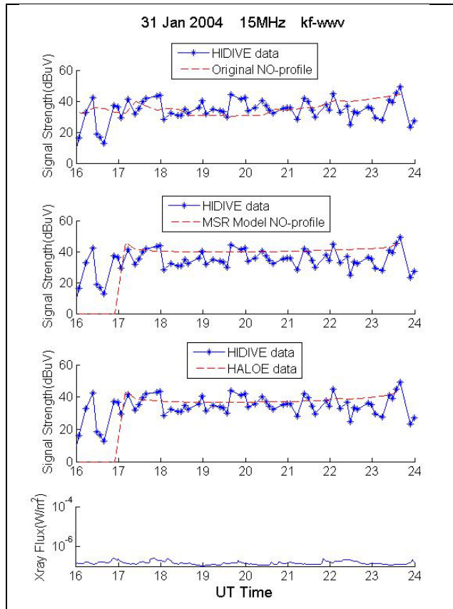
Figure F.11. HIDIVE data, GOES data, and AbbyNormal version predictions for the 15 MHz kf-wwv transmission on 31 January 2004.
