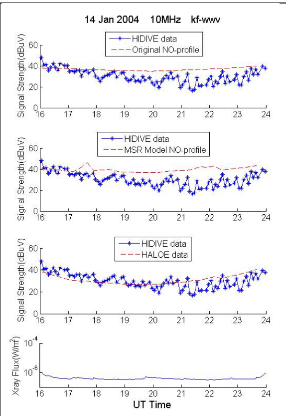
Figure E.4. HIDIVE data, GOES data, and AbbyNormal version predictions for the 10 MHz kf-wwv transmission on 14 January 2004.
