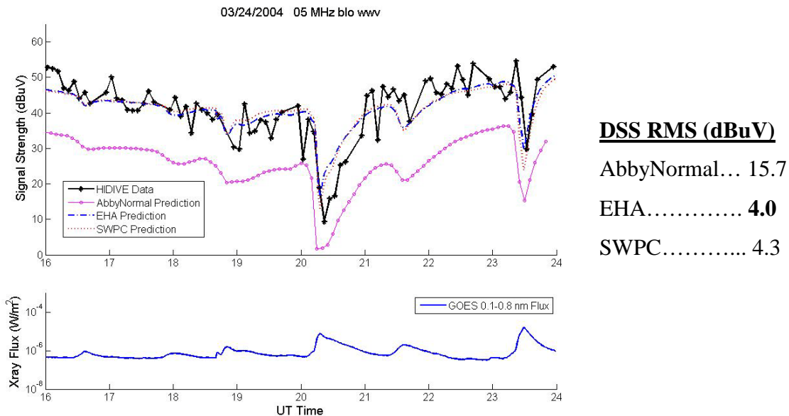
Figure 8.1.2. The AbbyNormal, EHA, and SWPC predictions for signal strength for the 5 MHz blo-wvw HIDIVE transmission on 24 March 2004.
