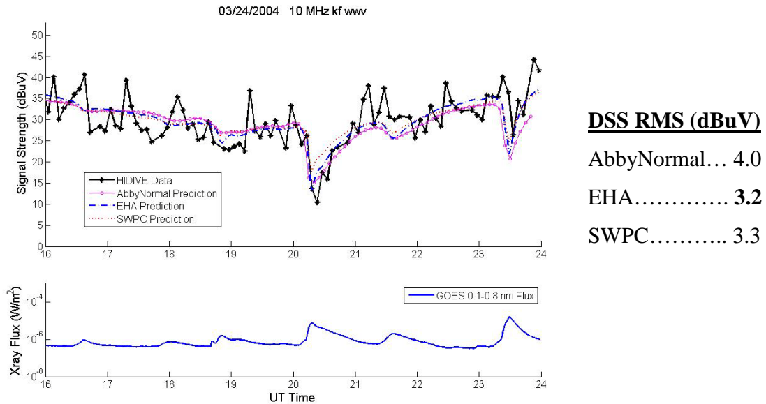
Figure 8.1.3. The AbbyNormal, EHA, and SWPC predictions for signal strength for the 10 MHz kf-wwv HIDIVE transmission on 24 March 2004.
