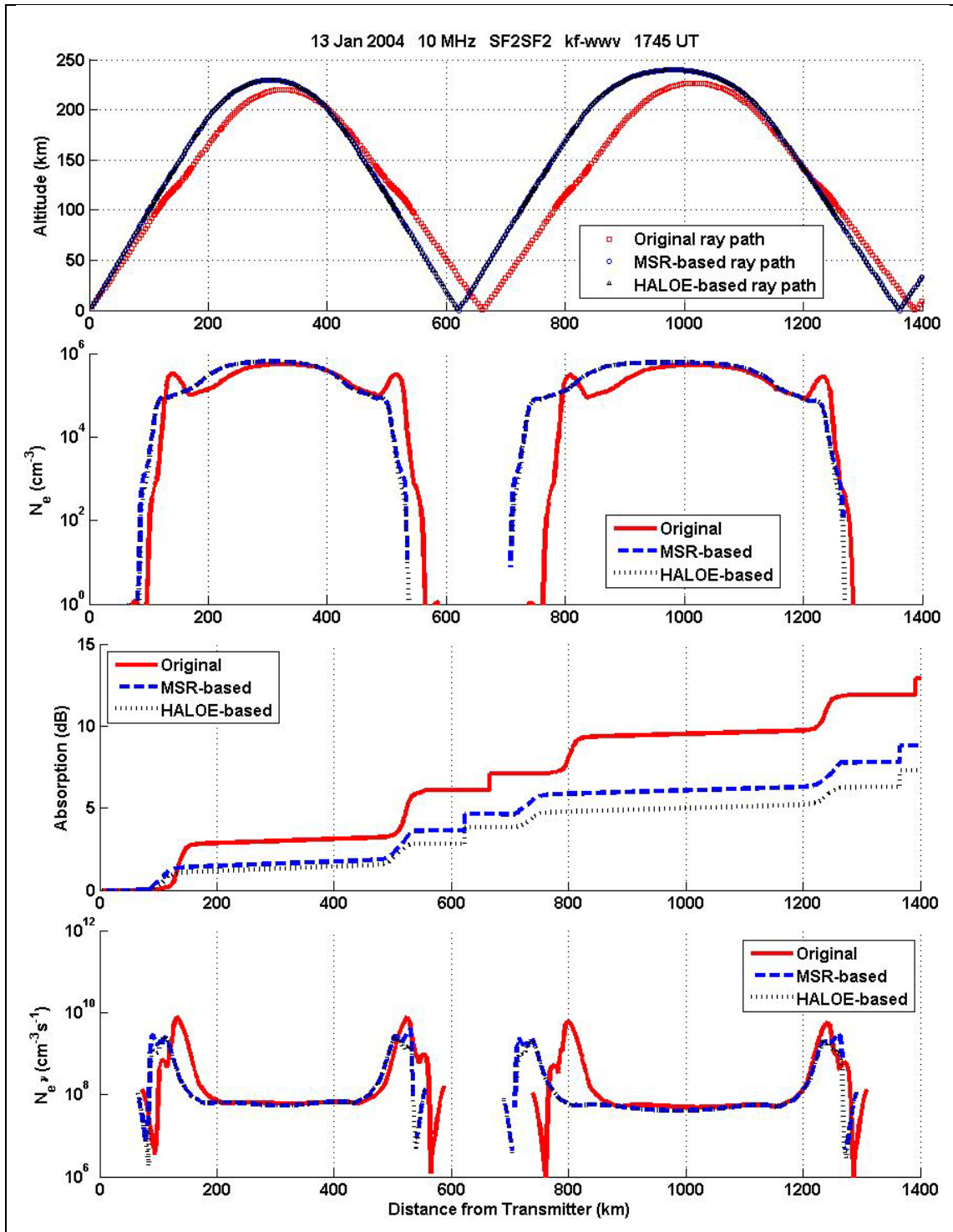
Figure 9.5.16. F-mode propagation paths predicted by HASEL for the 10 MHz kf-wwv transmission on 13 January 2004 at 17:45 UT are shown in the top panel. Also shown are the predictions of the three AbbyNormal versions of N_e along the raypath (second panel from top), total absorption suffered by the wave as it propagates (second panel from bottom), and N_e \nu along the raypath (bottom panel).
