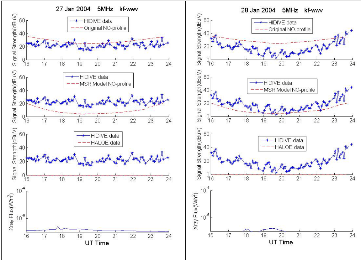
Figure D7. HIDIVE data, GOES data, and AbbyNormal version predictions for the 5 MHz kf-wwv transmission on 27 January 2004.
