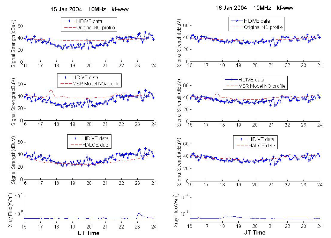
Figure E.5. HIDIVE data, GOES data, and AbbyNormal version predictions for the 10 MHz kf-www transmission on 15 January 2004.
