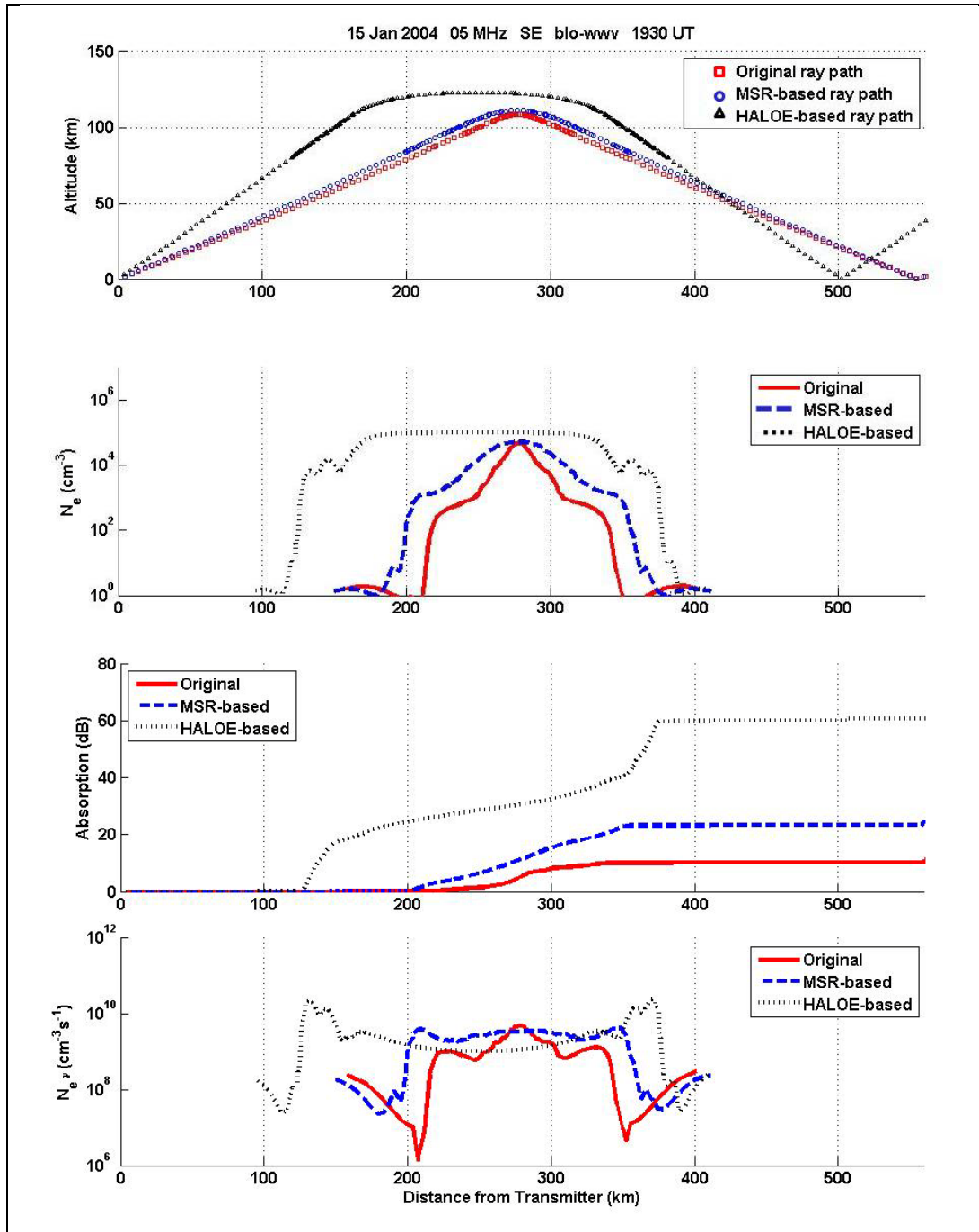
Figure 9.5.3. Dominant propagation paths predicted by HASEL for the 5 MHz blo-wwv transmission on 15 January 2004 at 19:30 UT are shown in the top panel. Also shown are the predictions of the three AbbyNormal versions for N_e along the raypath (second panel from top), total absorption suffered by the wave as it propagates (second panel from bottom), and N_e \nu along the raypath (bottom panel).
