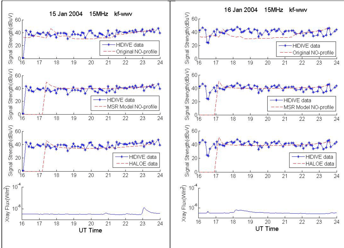
Figure F.5. HIDIVE data, GOES data, and AbbyNormal version predictions for the 15 MHz kf-wwv transmission on 15 January 2004.
