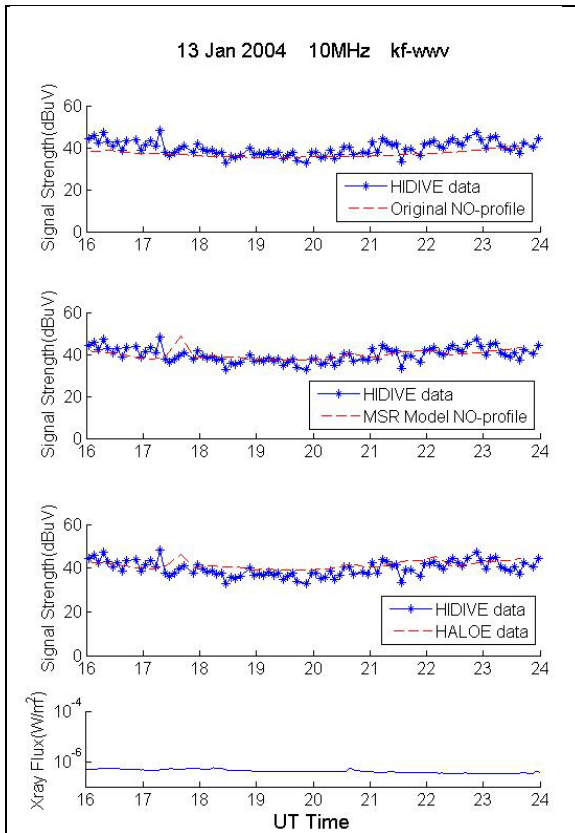
Figure E.3. HIDIVE data, GOES data, and AbbyNormal version predictions for the 10 MHz kf-wwv transmission on 13 January 2004.
