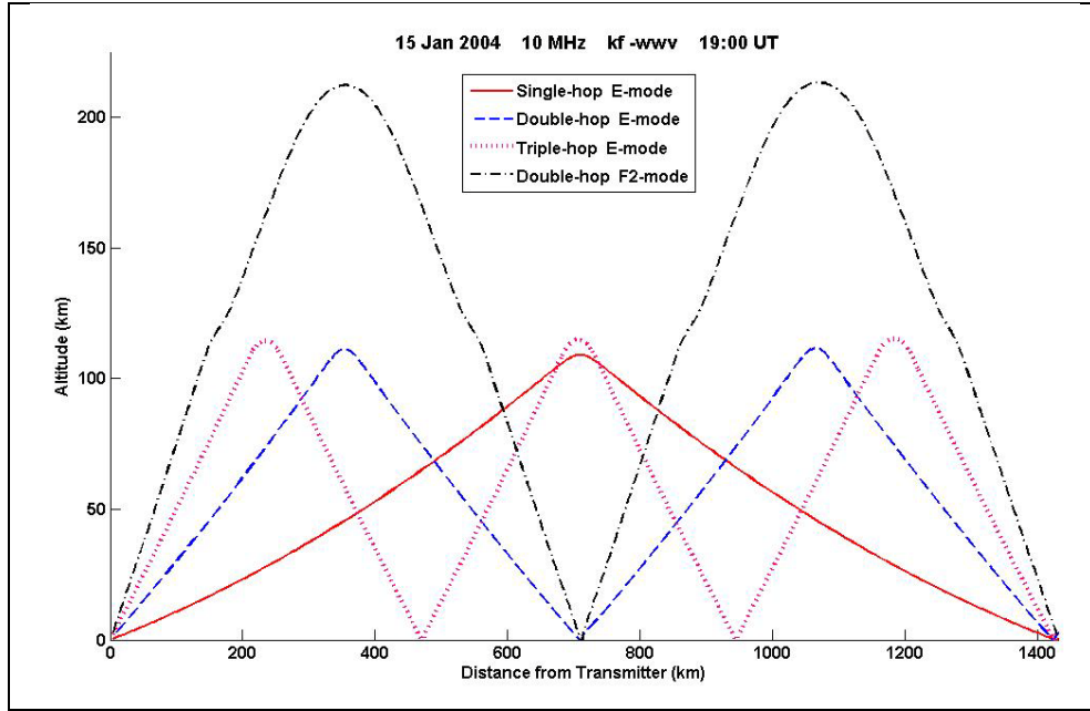
Figure 2.4.2. Various propagation modes available to a 10 MHz radio signal on 15 January 2004 at 19:00 UT transmitted from Fort Collins, Colorado to Klamath Falls, Oregon (ground distance of 1409 km), which include a single-hop E-mode, double-hop E-mode, triple-hop E-mode, and double-hop F2-mode.
